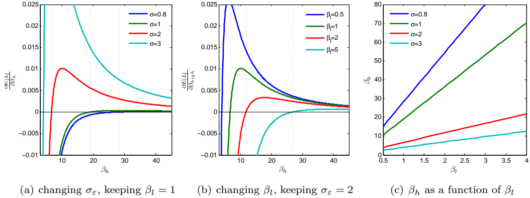
Figure 4: The relation between \beta_h and \beta_l in Rogoff's conservative banker setting.
