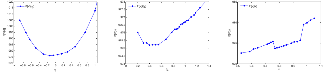
(a) keeping (\beta_h, \kappa) = (1, 0.8) , changing y_i^* (b) keeping (\kappa, y_i^*) = (0.8, 0) , changing \beta_h (c) keeping (\beta_h, y_i^*) = (1, 0) , changing \kappa
